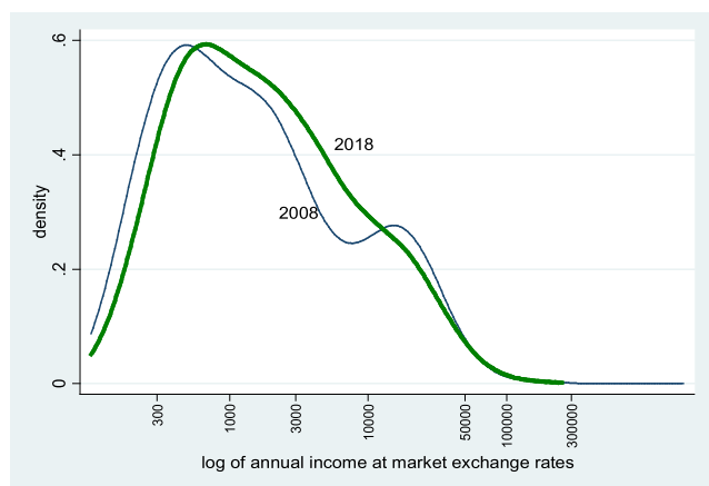
Fig. 4b. Global income distributions in 2008 and 2018 (income at MERs). Note: See Annex I. Both the coverage of the world population and of the world GDP is above 90 percent.
