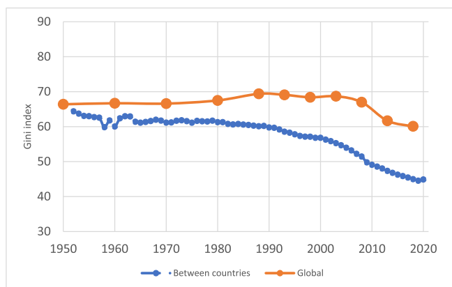
Fig. 3a. Global inequality and population-weighted inequality between countries (in PPP dollars, 1950–2018/20).
