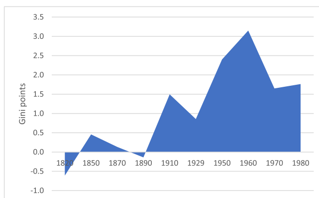
Fig. A2. Difference in calculated global inequality between the revised and the original Bourguignon-Morrison series (in Gini points). Note: The area shows the difference in Concept 3 inequality between the revised and original Bourguignon-Morrison data series.
