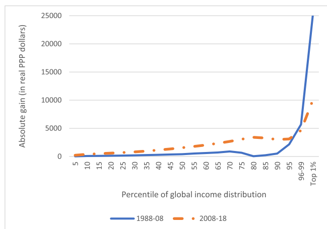
Fig. 5b. Global growth incidence curves for 1988–2008 and 2008–2018 (in absolute terms). Note: The fractiles are anonymous (that is, the global fractiles in 2018 are composed of country/percentiles that “fall” into that fractile in 2018 and which are normally different from the country/percentiles that were in that global fractile in 2008). The same holds for the period 1988–2008. For the distinction between anonymous and quasi non-anonymous growth in this context, see Lakner and Milanovic (2016). All incomes are expressed in PPPs.
