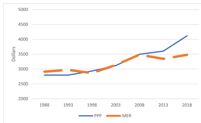
Fig. 9. Absolute Gini (for incomes at PPP dollars or at market exchange rate). Note: The figure shows one-half of the average income gap between two random individuals in the world when incomes are measured either in real international (PPP) dollars or dollars at the nominal market exchange rate deflated to 2011 US dollars.
