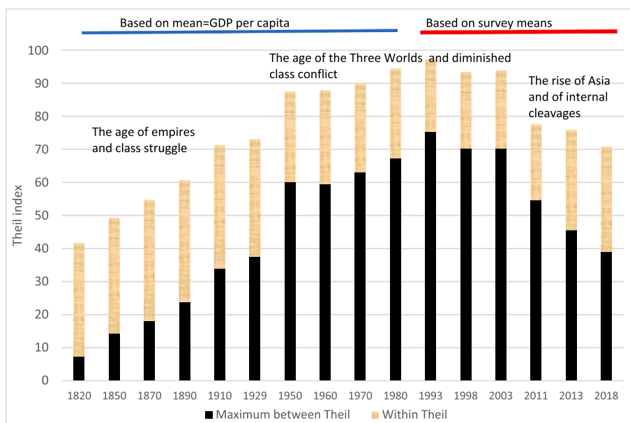
Fig. 2. Decomposition of global income inequality 1820–2018. (all in PPP dollars; mean income approximated by GDP per capita up to 1980 and by household survey mean afterwards). Note: 1820–1980 based on the revised Bourguignon and Morrison (2002) data series; 1993–2008 based on Lakner and Milanovic (2016); 2008–13 based on Milanovic (2022); 2018, unpublished results. For more detail, see Annex I. The horizontal line on the top indicates that the data on the left are based on country mean incomes approximated by GDP per capita, and the data on the right on the means derived from household surveys.
