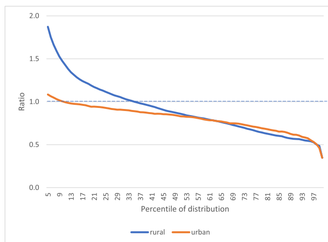
Fig. A4. Consumption vs income levels at equivalent percentiles of rural and urban distributions. Note: Value greater than 1 means that consumption levels are greater than income levels (at equivalent percentiles of the distribution). Consumption data from Sinha Roy and van der Weide (2022); income data extrapolated from the 2011 survey.
