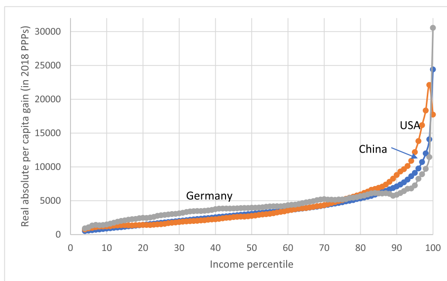
Fig. 6b. Absolute income gains by percentile for China, US and Germany, 2007/08 to 2018 (in 2018 PPP dollars). Note: Calculated from LIS data for US and Germany for 2008 and 2018, and LIS data for China 2018 and CHIP for China 2007. Nominal amounts deflated by countries' Consumer Price Indices to obtain real growth rates shown in Fig. 6a. Real absolute income gains in domestic currency normalized by 2018 PPPs to obtain the gains in Fig. 6b.
