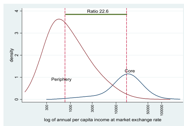
Fig. 11b. Distribution of income in the core and periphery countries in 2018 (incomes in dollars at market exchange rate). Note: Core is defined as Western Europe, North America, Oceania and Japan. Periphery is defined as all other countries except China. The vertical dashed lines are drawn at the points of median incomes. The areas under the curves reflect population sizes.
