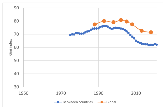
Fig. 3b. Global inequality and population-weighted inequality between countries (at market exchange rates, 1975–2021). Note: The between-country inequality calculated from GDPs per capita and population sizes available in World Bank Development Indicators database.
