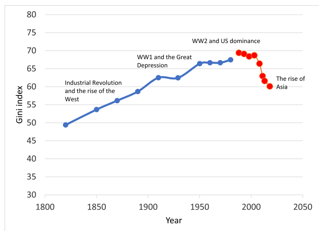
Fig. 1. Estimated global income inequality 1820–2018 (incomes in PPP dollars). Note: 1820–1980 based on the revised Bourguignon and Morrisson (2002) data series; 1988–2008 based on Lakner and Milanovic (2016); 2008–13 based on Milanovic (2022); 2018, unpublished results. For fuller explanation see Annex I and Annex IV. The Figure shows the break in the data sources between the series where country means are GDP per capita (up to 1980 and following the work by Bourguignon and Morrisson) and the series where country means are derived from household surveys (after 1988).
