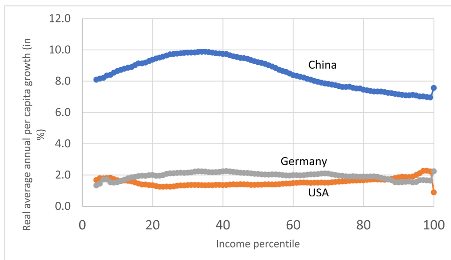
Fig. 6a. Growth rates across income distributions for China, US and Germany, 2007/08 to 2018.
