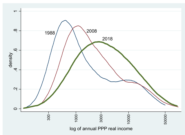
Fig. 4a. Global income distribution in 1988, 2008 and 2018 (income in PPP dollars).
